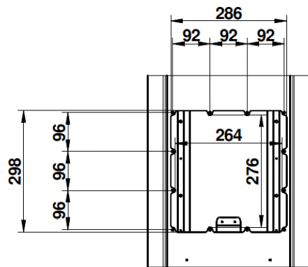
Detail D
